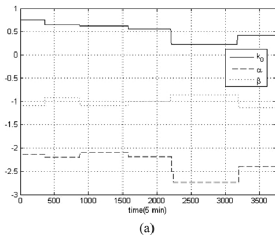
Fig. 6. Values of k_0 , \alpha and \beta used in MI models during grade change operations: (a) Case A, (b) Case B.
