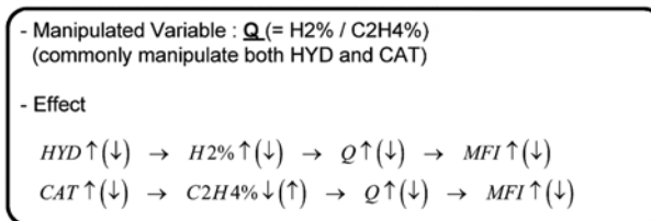
Fig. 15. MI control specification.
